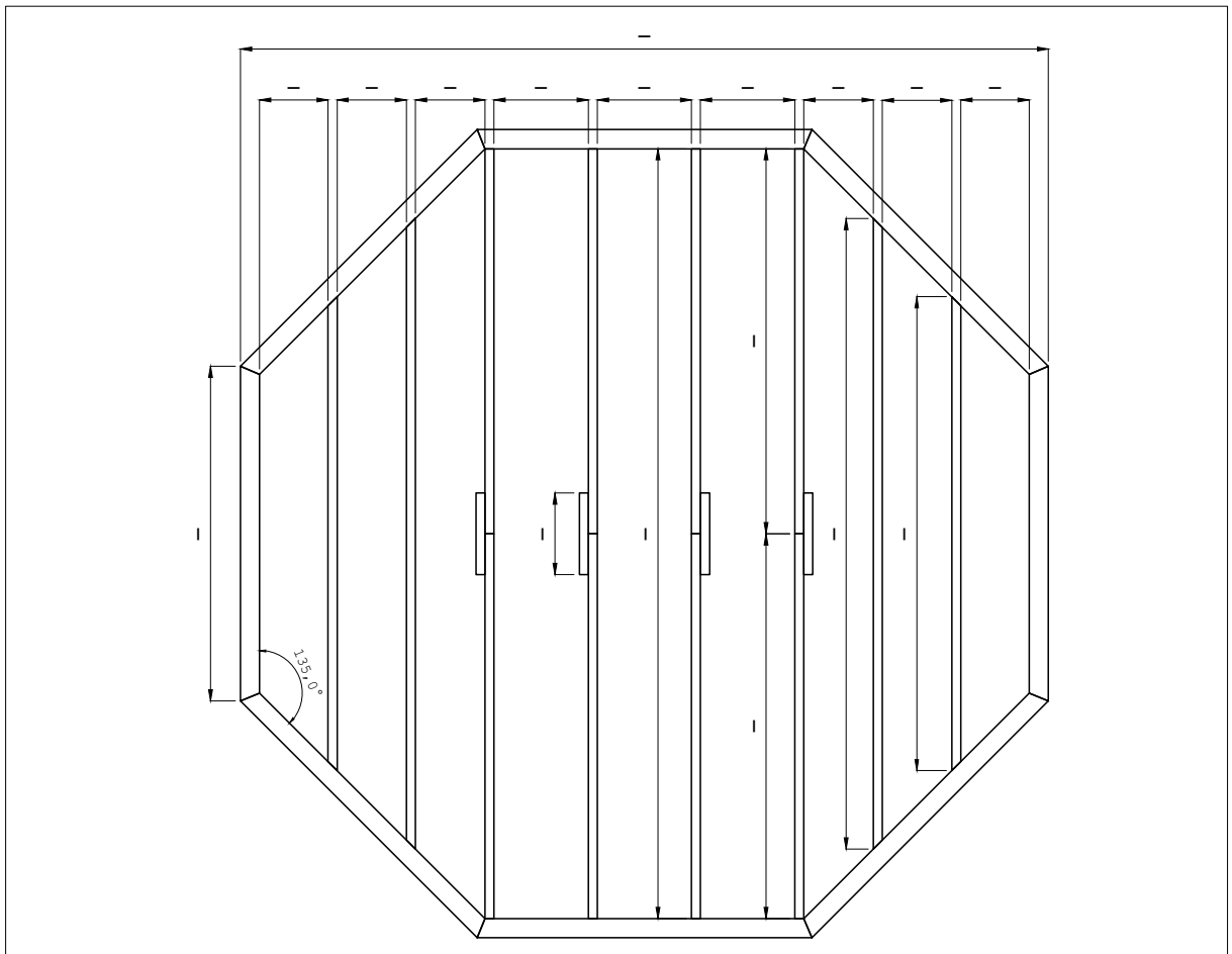
Fundamentplan 1
